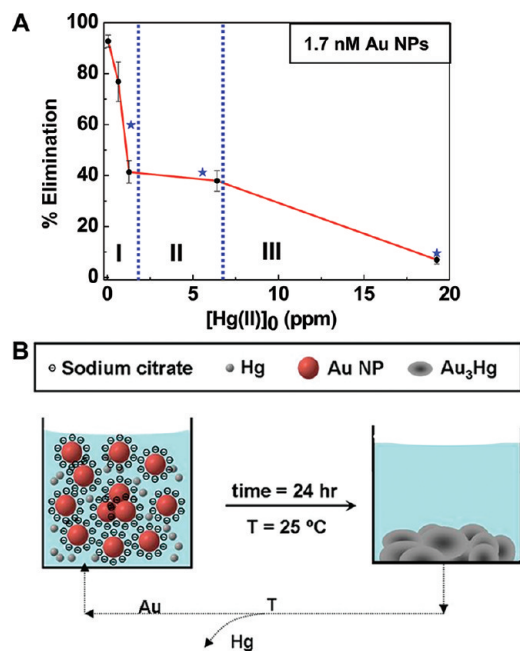
Figure 1. Removal of Hg by Au NPs from water solutions. (A) Percentage of elimination of Hg(II) employing a constant Au NP concentration (1.7 nM Au NPs, 7.1 ppm Au) from samples containing increasing initial HgCl 2 concentrations in Milli-Q water (circles with error bars) or in river water (stars). All the concentrations refer to the total amount in the reaction vessel. (B) Schematic representation of the Hg(II) elimination process through amalgam formation (not drawn to scale). The recovery of Hg and Au from the amalgam is a well-known and extended process.
